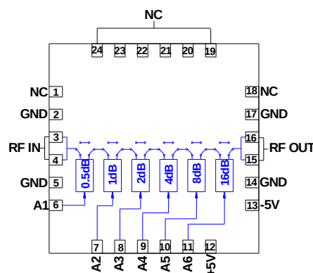
Functional Diagram
